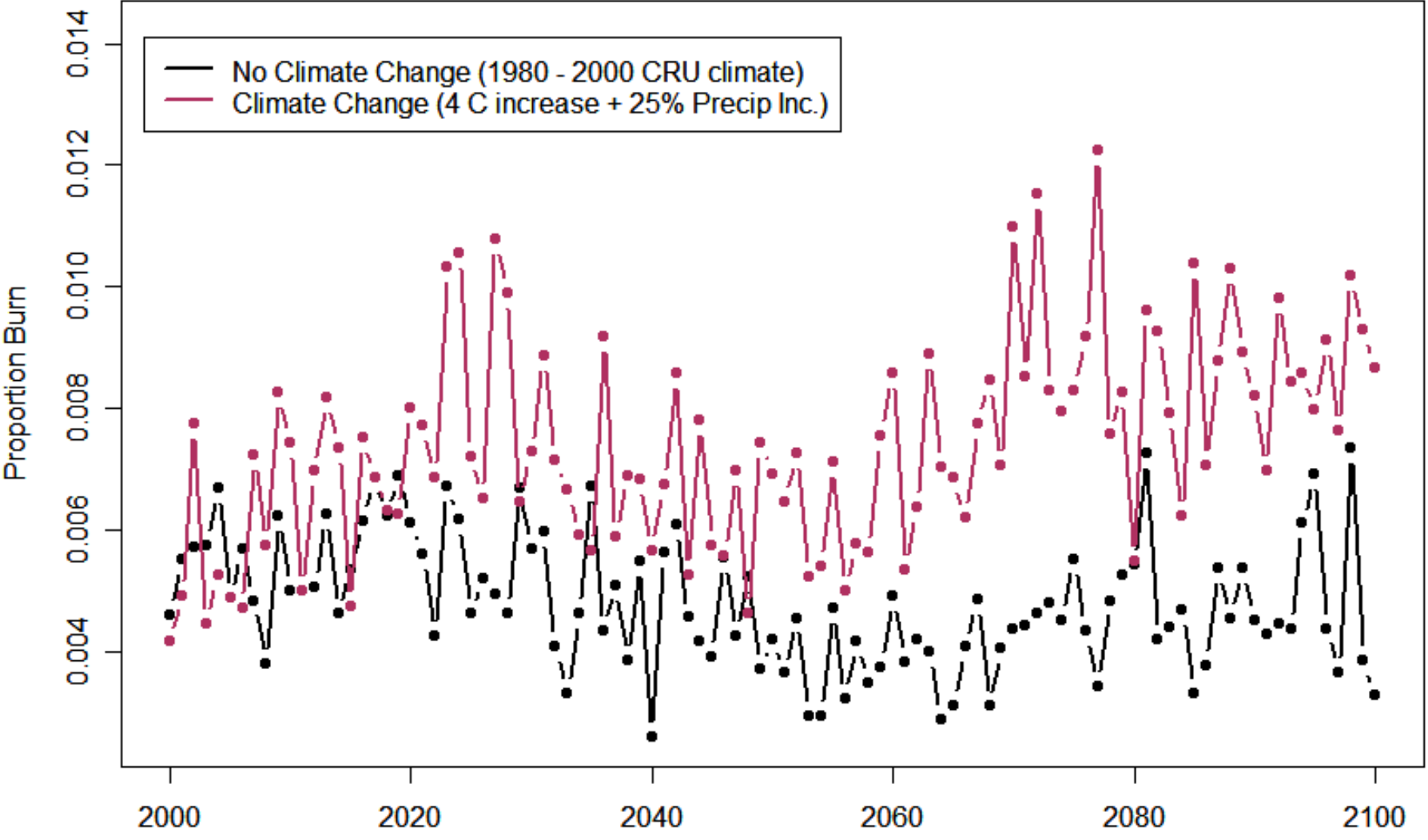
Proportion of Landscape Burn -- Average across 100 Reps
