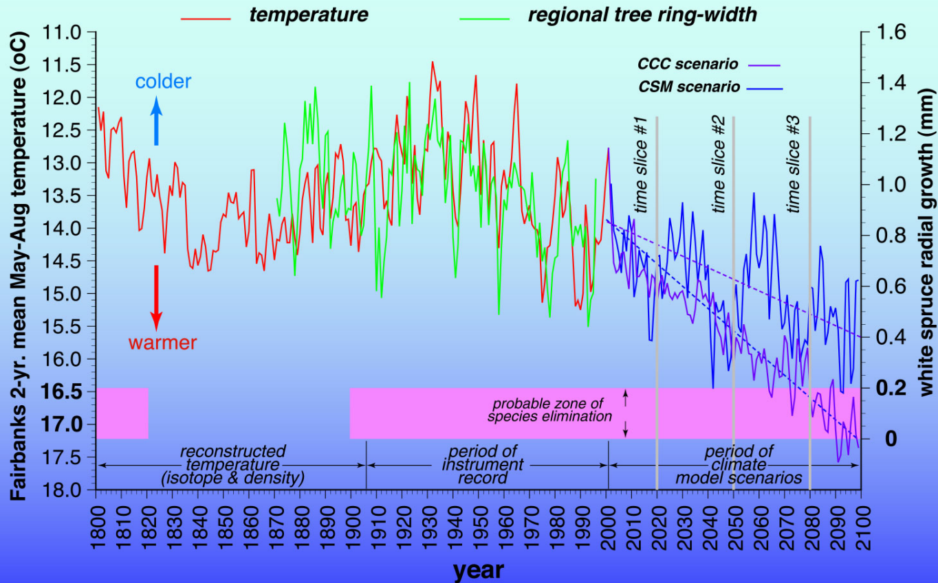
Historic and reconstructed relationship between white spruce growth and summer temperature and climate scenarios in central Alaska
